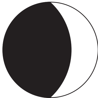
Waxing Crescent
