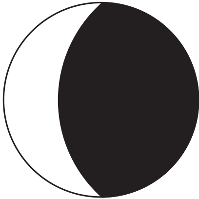
Waning Crrescent
