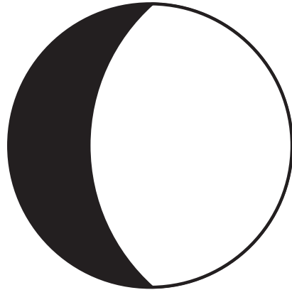
Waxing Gibbous
