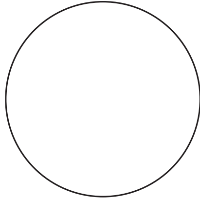
Full Moon
