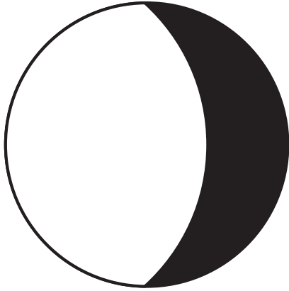
Waning Gibbous
